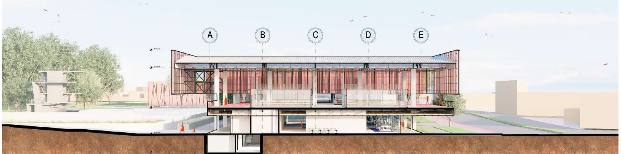
CORTE TRANSVERSAL C3-C3
