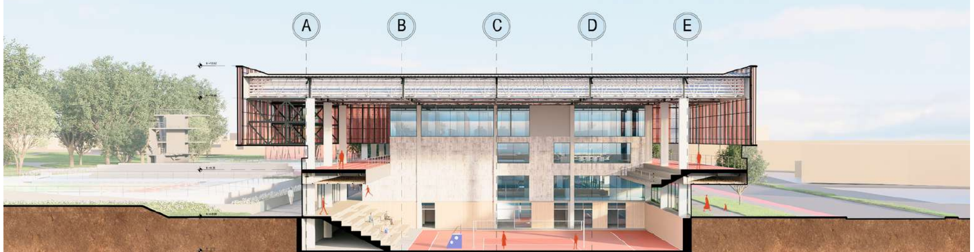
CORTE TRANSVERSAL C3-C3
