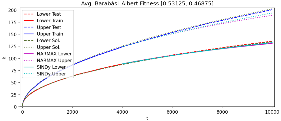
Figure 9.11: Estimations of the SINDy and NARMAX methods from the identified model of the initial node from the BA Fitness model with discrete fitness levels [0.53125, 0.46875] averaged over 100 realisations.
