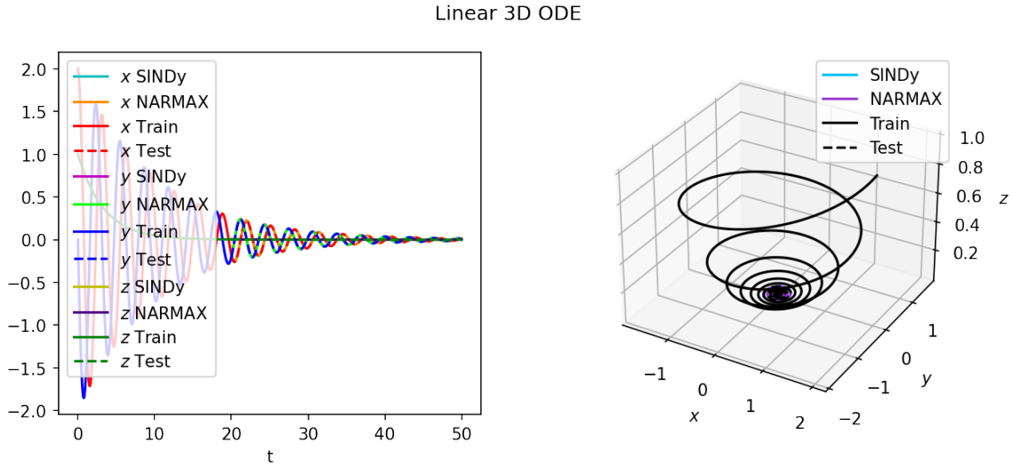
Figure 9.3: Estimations from the SINDy and NARMAX methods of the Linear 3D ODE from equations 5.3.
