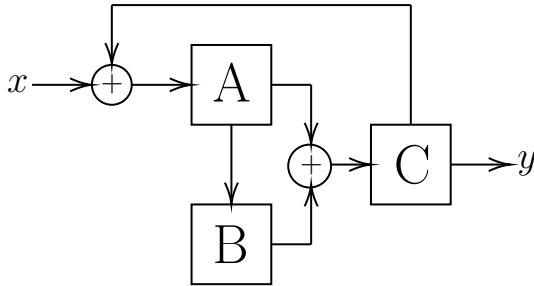
Figure 3.1: State-Space Representation example of a system with three state variables, an input x and output y , related by equations 3.1 .
