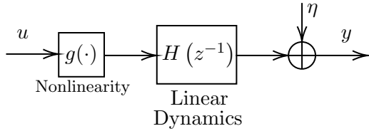
Figure 4.1: Hammerstein Model
