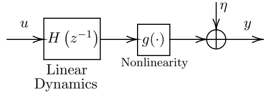
Figure 4.2: Wiener Model
