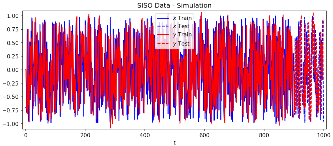
Figure 5.4: Example of the nonlinear function 5.6 where x is a uniform random variable.
