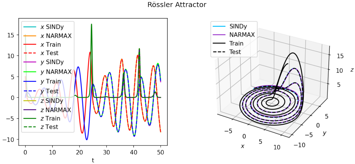
Figure 9.5: Estimations from the SINDy and NARMAX methods of the Rössler Attractor from equations 5.5.
