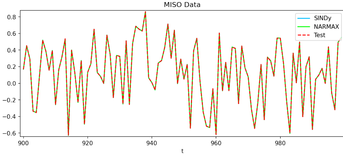
Figure 9.7: Estimations from the SINDy and NARMAX methods of the MISO function from equation 5.7 .
