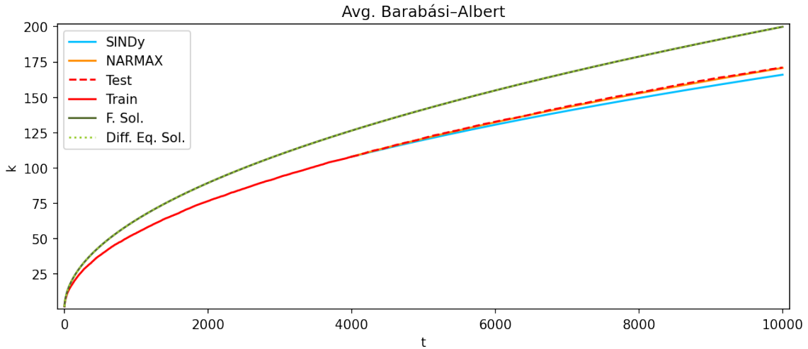
Figure 9.8: Estimations of the SINDy and NARMAX methods from the identified model of the initial node from the BA model averaged over 100 realisations.
