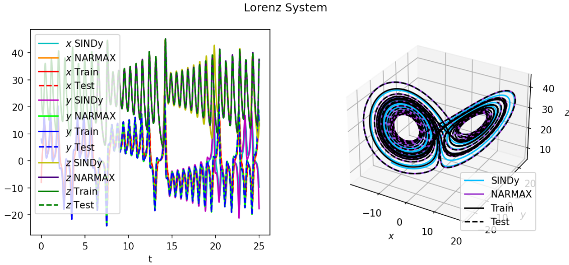
Figure 9.4: Estimations from the SINDy and NARMAX methods of the Lorenz system from equations 5.4.
