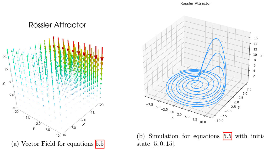
Figure 5.3: Rössler Attractor visualisations
