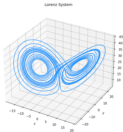
(d) Simulation for equations 5.4 with initial state [-8, 8, 27] .
