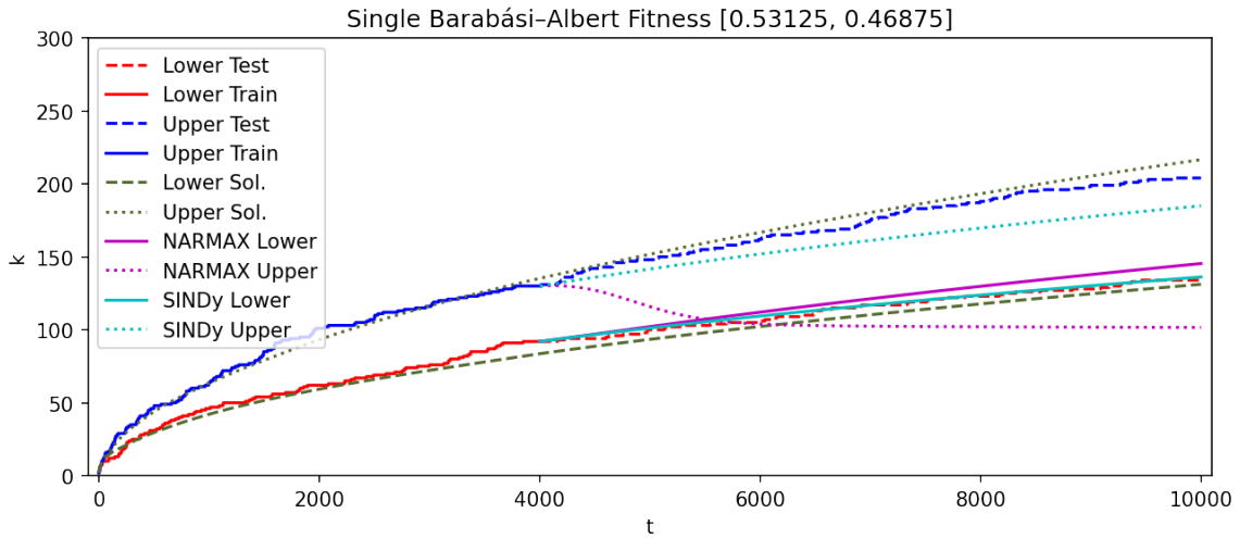
Figure 9.12: Estimation from the SINDy and NARMAX methods of the BA Fitness model with discrete fitness levels [0.53125, 0.46875] .
