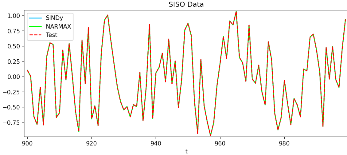
Figure 9.6: Estimations from the SINDy and NARMAX methods of the SISO function from equation 5.6.
