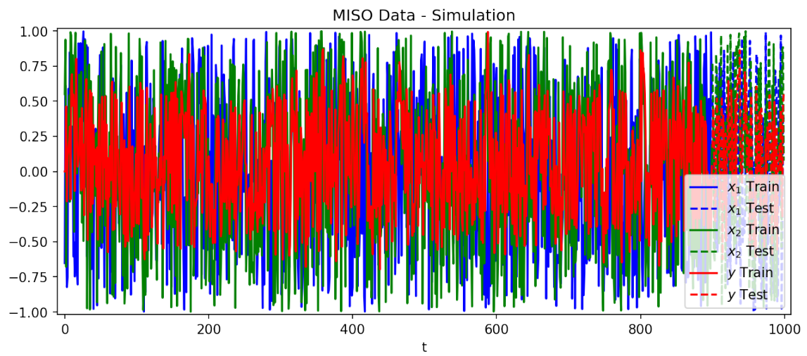
Figure 5.5: Example of the nonlinear function 5.7 where x is a uniform random variable.
