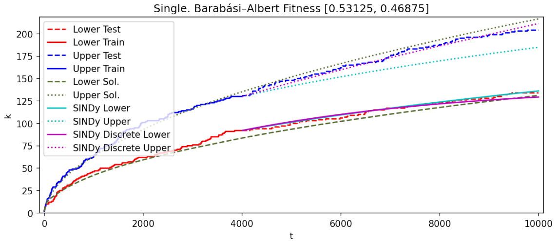
Figure 9.13: Estimation from the SINDy and NARMAX methods of the BA Fitness model with discrete fitness levels [0.53125, 0.46875] and SINDy in discrete mode.
