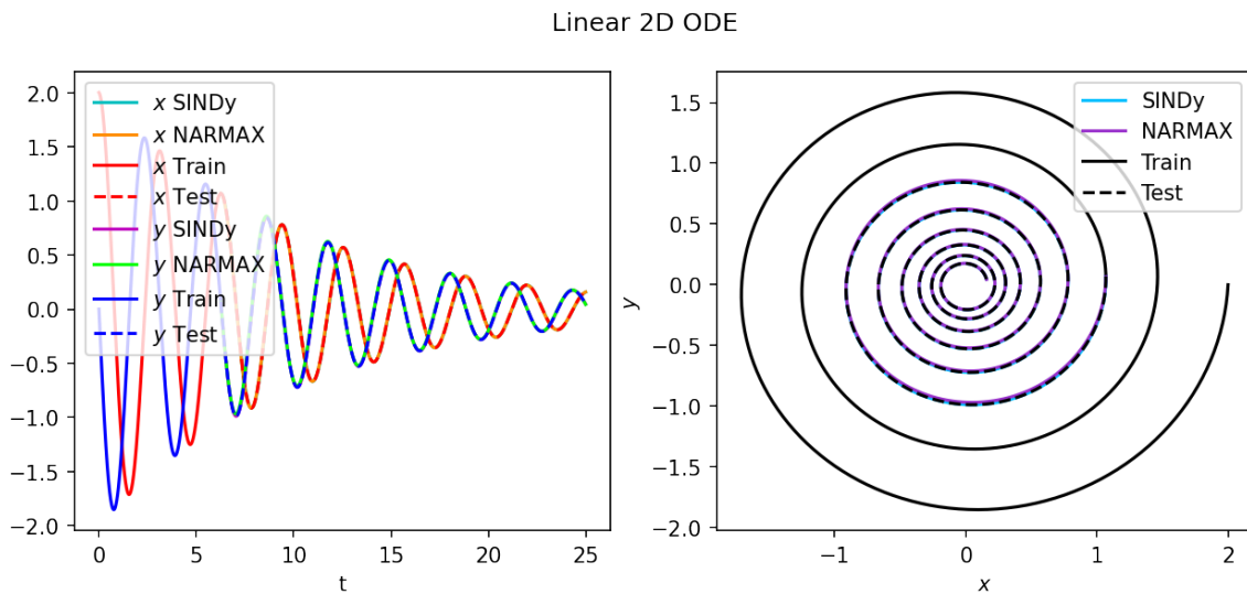
Figure 9.1: Estimations from the SINDy and NARMAX methods of the Linear 2D ODE from equations 5.1.
