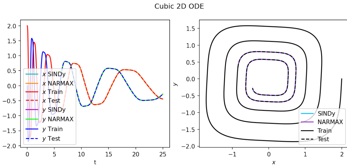
Figure 9.2: Estimations from the SINDy and NARMAX methods of the Cubic 2D ODE from equations 5.2 .
