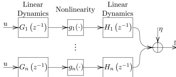
Figure 4.4: Parallel cascade general block-structured model with noise
