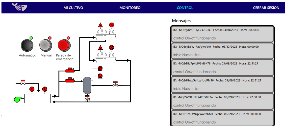
Figura 3.77: Vista final control
