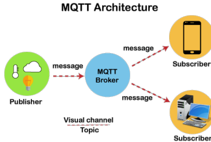
Figura 3.80: Arquitectura general MQTT [67]
